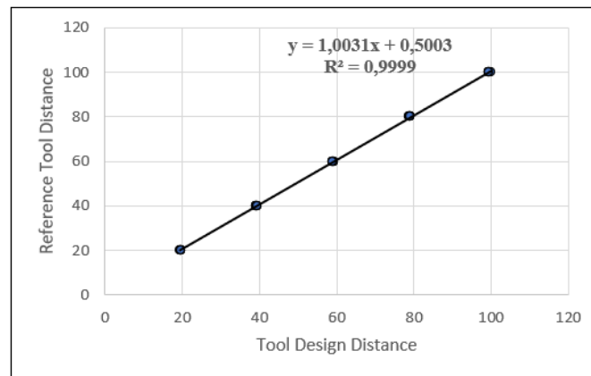
Fig. 6. Graph of distance parameter calibration
