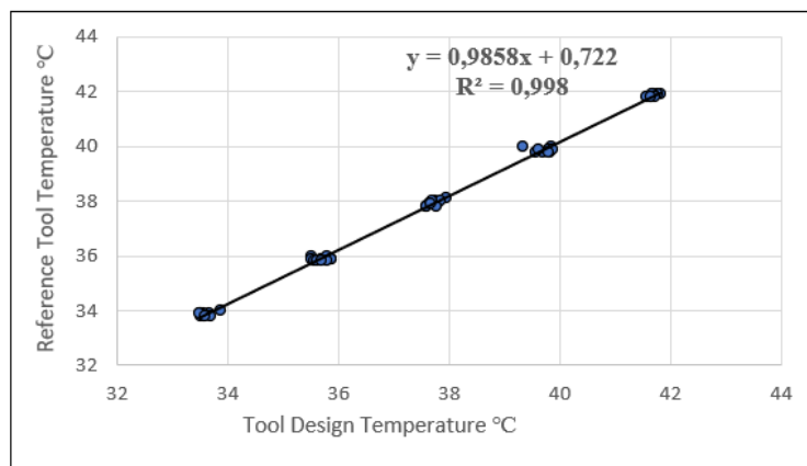
Fig. 4. Graph of temperature parameter calibration
