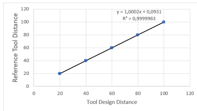
Fig. 7. The calibration graph of the distance parameter adjusted to the standard
