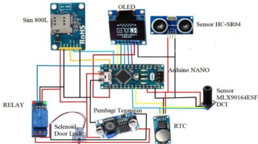
Fig. 2. Design of a series of tools
