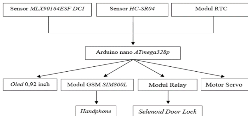
Fig. 3. Block diagram of measuring instrument design
