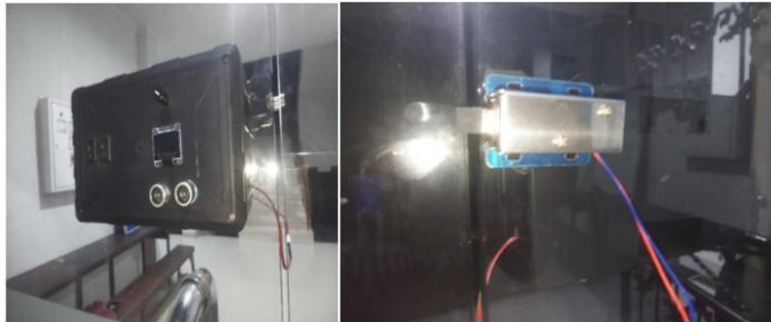
Fig. 1. Automatic door lock based on ATmega328P microcontroller with MLX90614ESF DCI and HC-SR04 sensors
