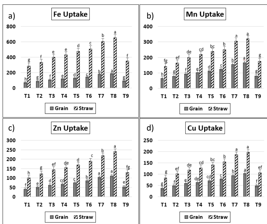
Fig. 2. Effect of different recommendation of fertilizer application approaches on a) iron, b) manganese, c) zinc and d) copper uptake ( \text{g ha}^{-1} ) by wheat. Bars with similar lowercase letters are not significantly different with respect to least significant difference (LSD) values at p=0.05
