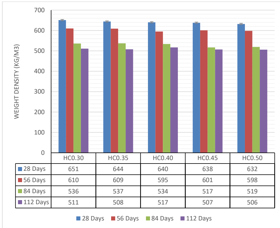
Fig. 5. Demonstrate the weight density of hempcrete at different days
