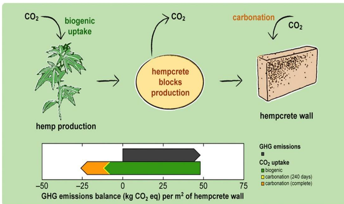
Fig. 10. Illustration of the carbon emissions and sequestration of hempcrete, showcasing a net emissions balance that demonstrates carbon negativity
