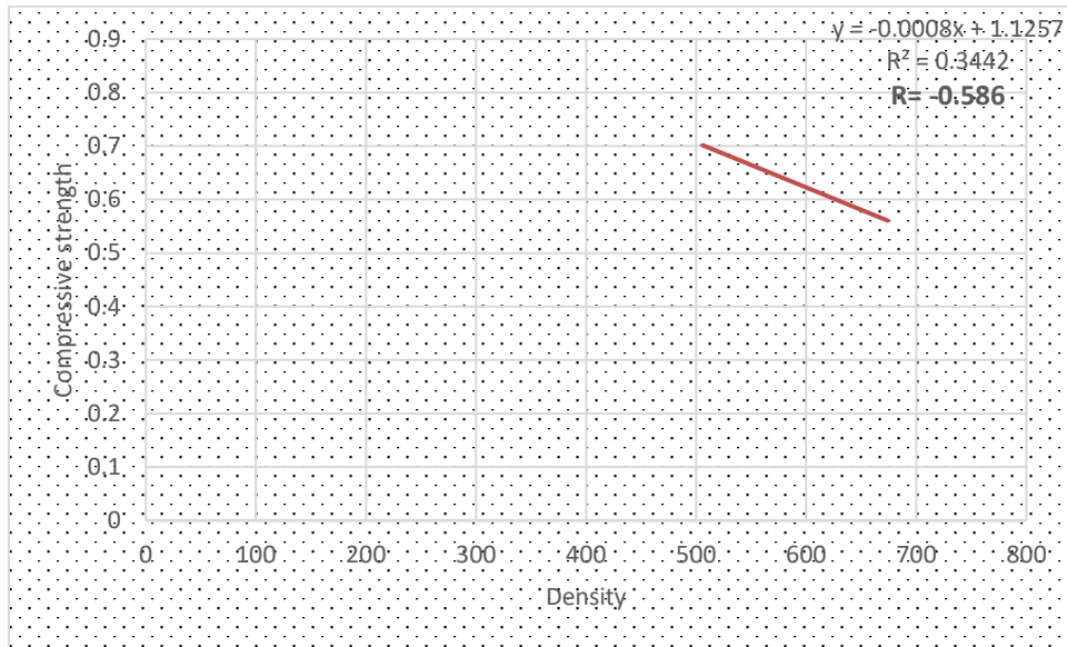
Fig. 8. Correlation between density and compressive strength
