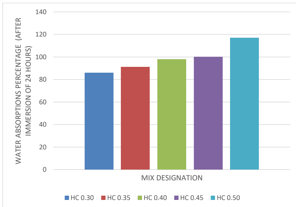
Fig. 6. Water absorptions of hempcrete
