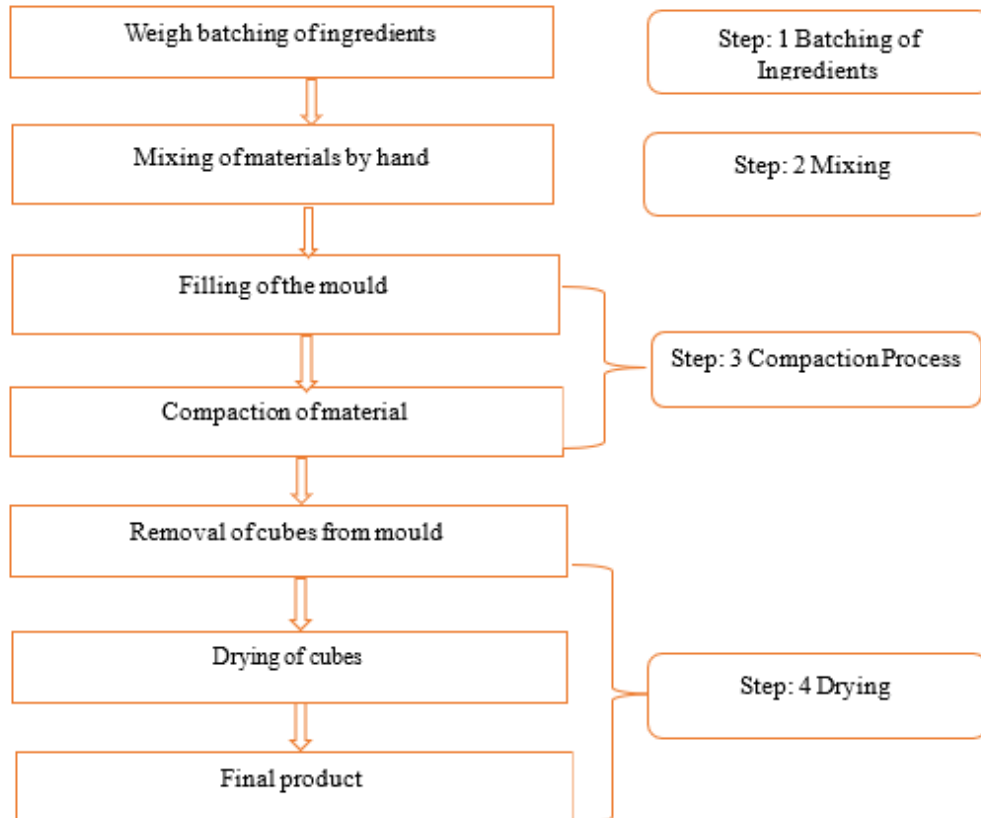
Fig. 3. Flow chart for the preparation of hempcrete
