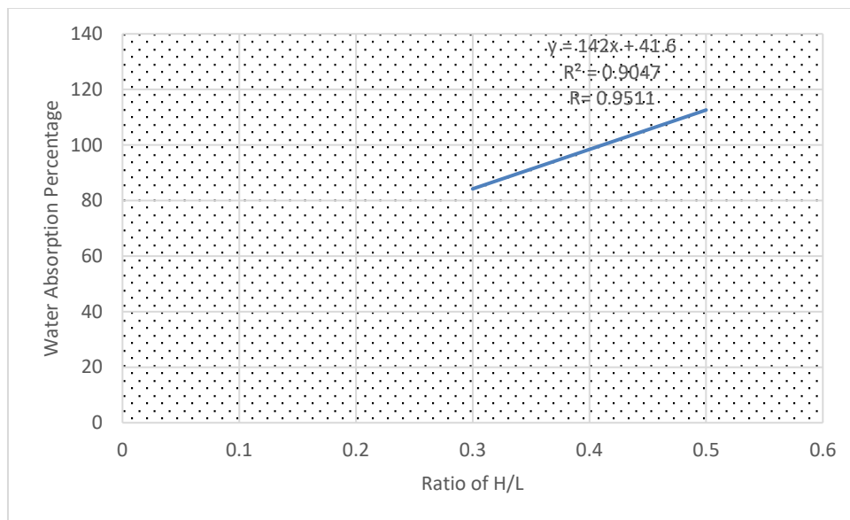
Fig. 9. Correlation between hemp-lime ratios and water absorption percentage
