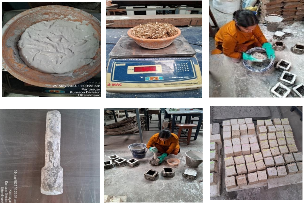
Fig. 4. Pictorial presentation of preparation of hempcrete; (a) slaked lime paste (b) weight batching of shiv (c) mixing of lime and shiv (d) iron rod used for compaction (e) compaction of concrete into the cube mould (f) Final view of hempcrete cubes
