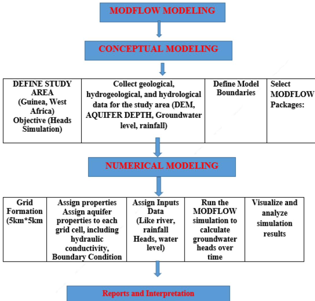
Fig. 2. Work flow chart of MODFLOW processing
