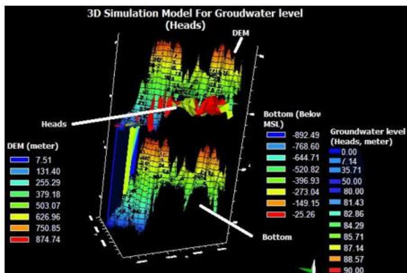
Fig. 6(b). Numerical 3D model of Modflow simulation of the Groundwater levels (Heads) Guinea (West Africa) region
