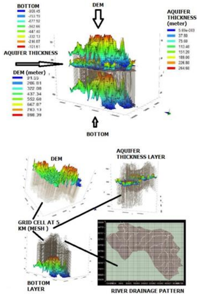
Fig. 6(a). Conceptual 3D model of Modflow simulation of the Guinea (West Africa) region
