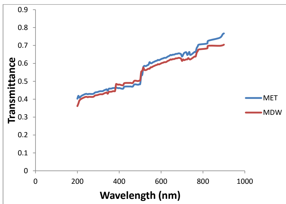
Fig. 3. Plot of transmittance against wavelength
