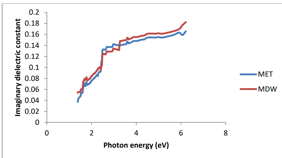
Fig. 9. Plot of Imaginary dielectric constant against photon energy
