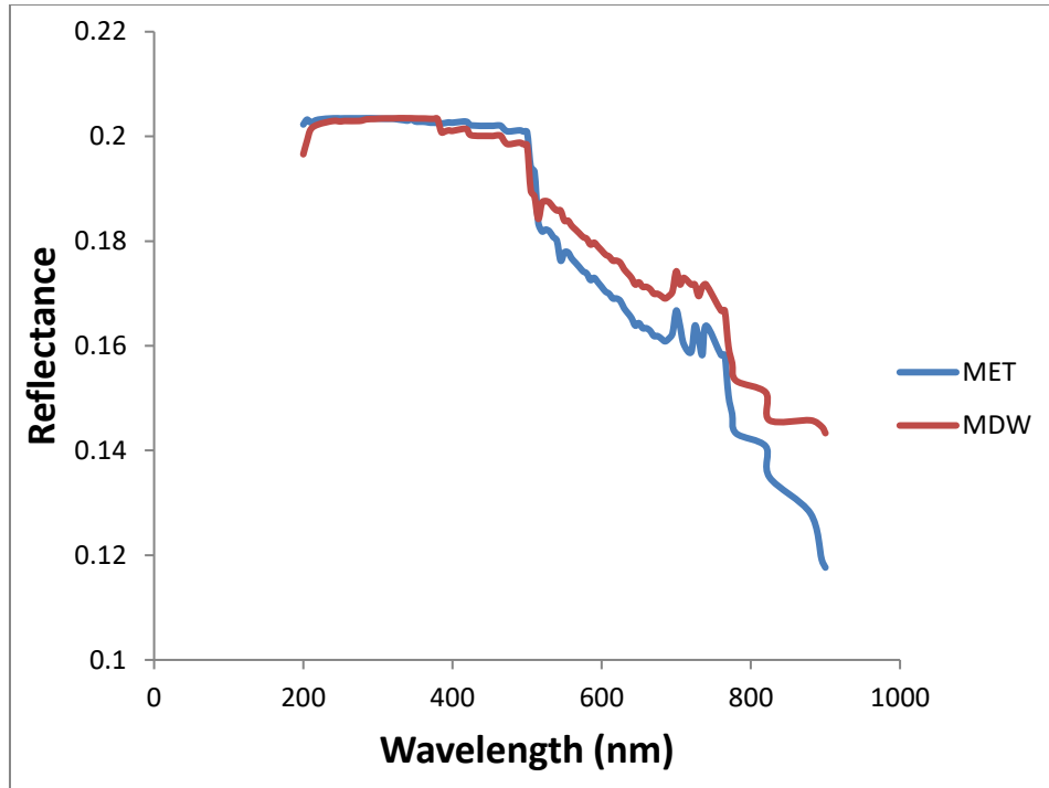
Fig. 4. Plot of reflectance against wavelength
