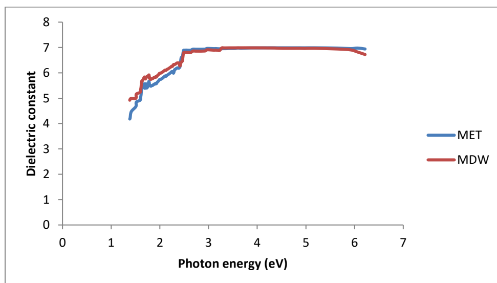
Fig. 8. Plot of Real Dielectric Constant against photon energy
