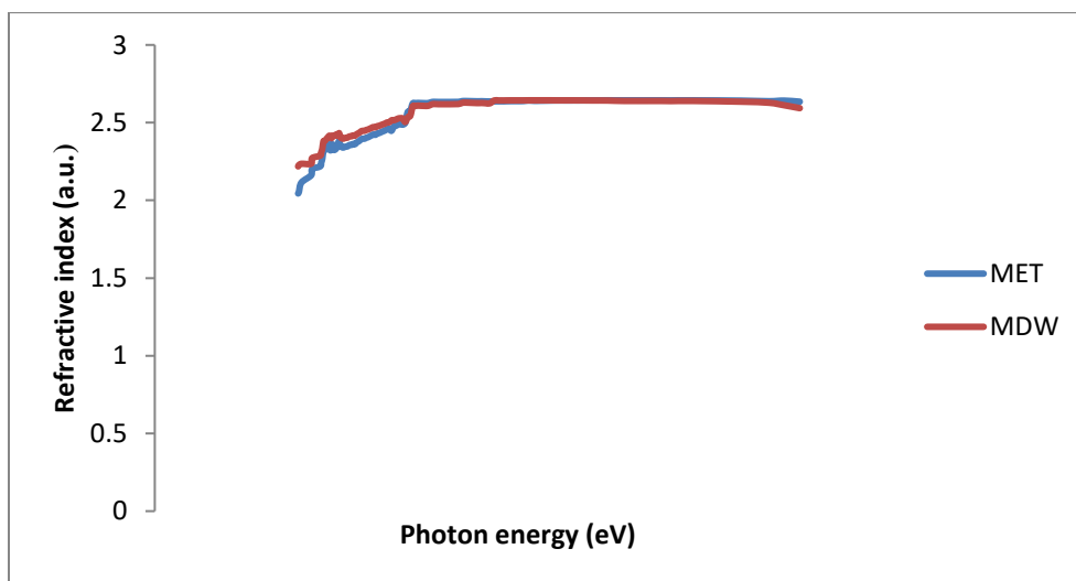
Fig. 5. Plot of refractive index against photon energy
