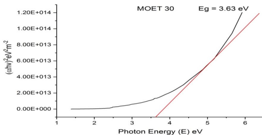
Fig.11. Plot of the band energy gap for monzaitite dispersed in ethanol
