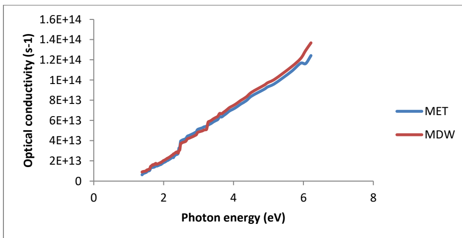
Fig. 10. Plot of Optical Conductivity against photon energy
