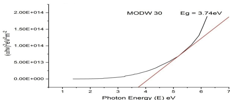
Fig. 12. Plot of the band energy gap for monazite dispersed in distilled water
