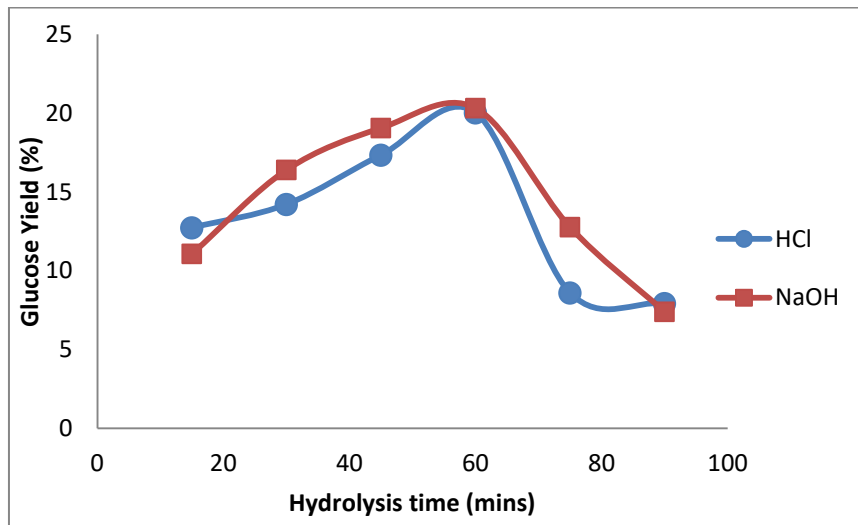
Fig. 6. Effect of hydrolysis time on yield of glucose using 2hr HCl and NaOH pretreated clay catalysts
