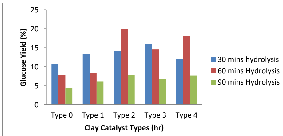
Fig. 7. Effect of acid activation times on hydrolysis using 0.06g/30ml catalyst dosage each
