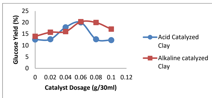
Fig. 3. Effect of catalyst dosage on hydrolysis using 2 hr HCl and NaOH activated clays for 60 minutes hydrolysis reaction time
