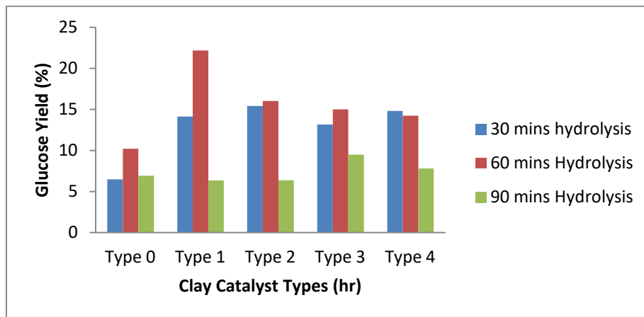
Fig. 8. Effect of alkaline activation times on hydrolysis using 0.04g/30ml catalyst dosage each
