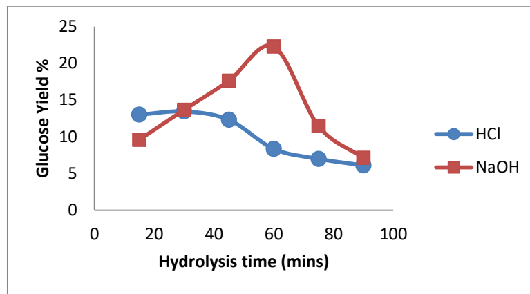
Fig. 5. Effect of hydrolysis time on yield of glucose using 1hr HCl and NaOH pretreated clay catalysts
