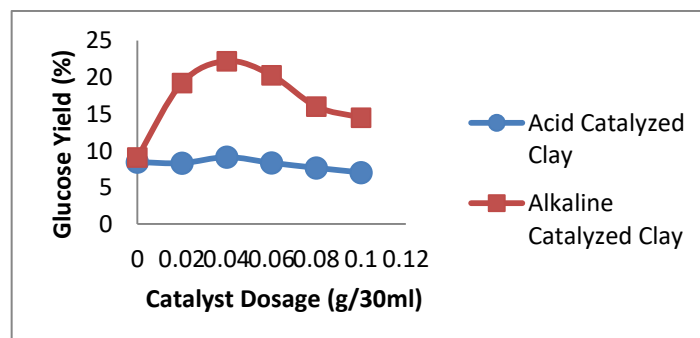
Fig. 2. Effect of catalyst dosage on hydrolysis using 1 hr HCl and NaOH activated clays for 60 minutes hydrolysis reaction time
