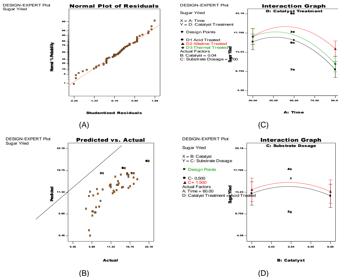
Fig. 9. Predicted and Actual plots, and interaction graphs of substrate and catalyst dosages, time, and catalyst treatment
