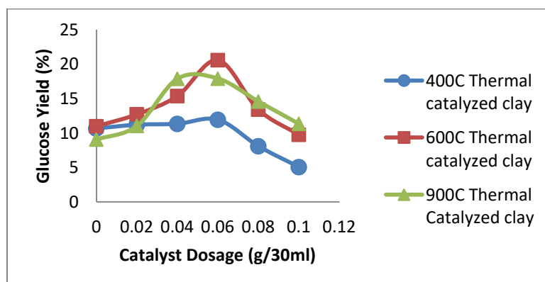
Fig. 4. Effect of catalyst dosage on hydrolysis using thermally activated clay at 400°C, 600°C, and 900°C for 60 minutes hydrolysis reaction time
