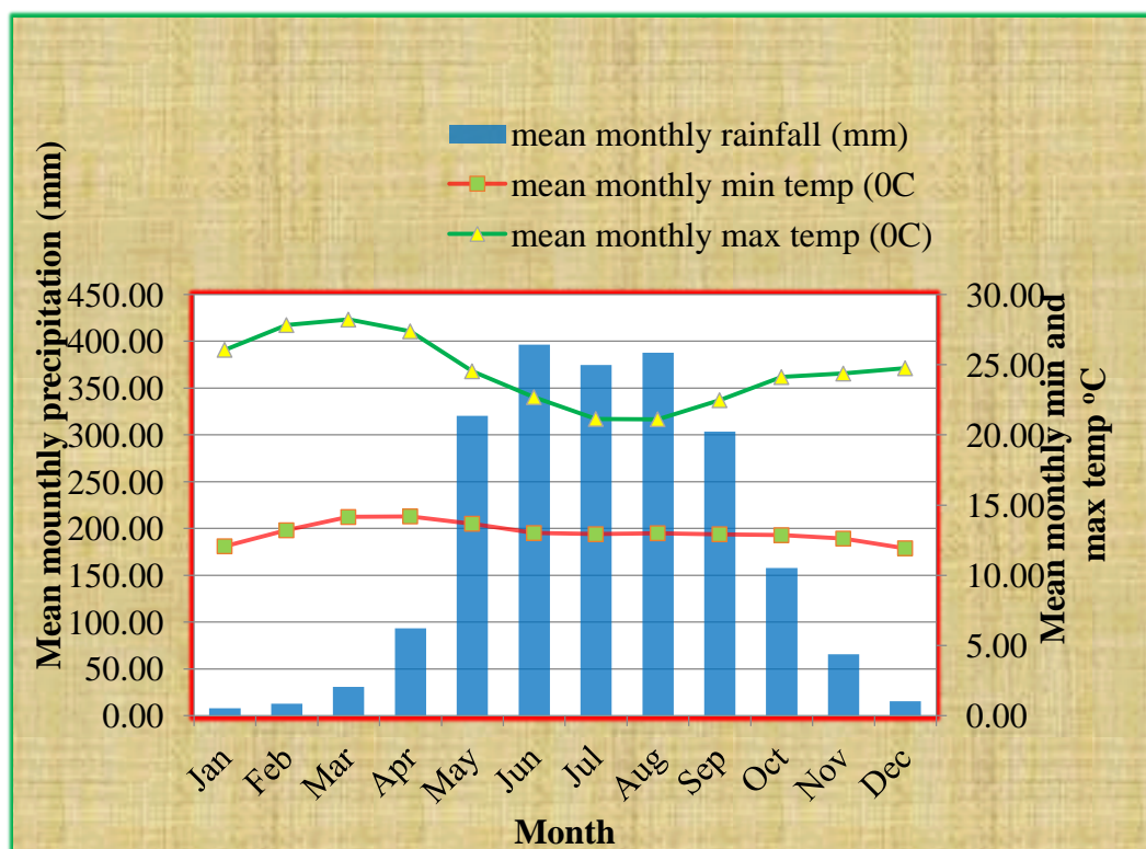
Fig. 2. Mean monthly rainfall, maximum and minimum temperatures of the study area for the years 2006 – 2018. (Nekemte Meteorological Station)
