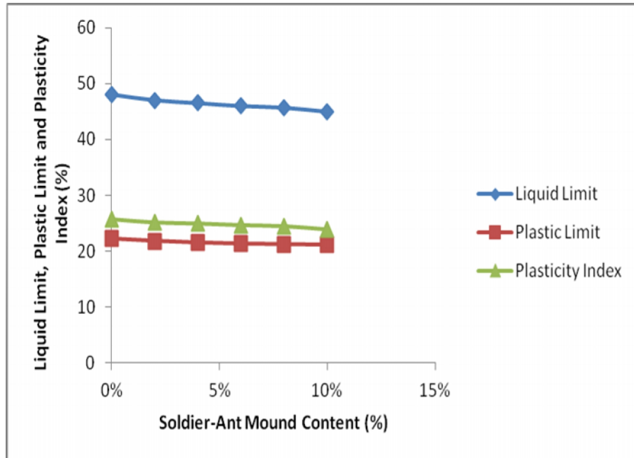
Fig. 2. Variation of liquid limit, plastic limit and plasticity index with soldier-ant mound content
