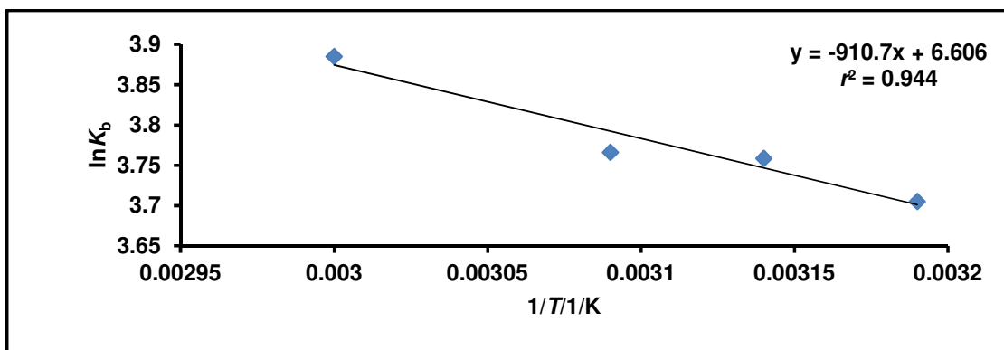
Fig. 5. van't Hoff plot for the determination of enthalpy of calcium ion binding to sites apart from intrinsic sites
