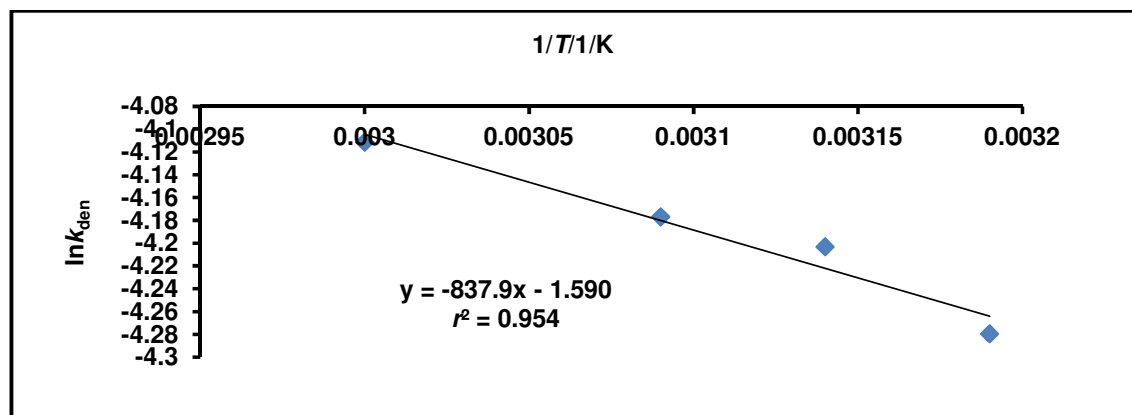
Fig. 4. Arrhenius plots for the determination of activation energy for the unfolding of the enzyme as [CaCl_{2(aq)}] \rightarrow 0
