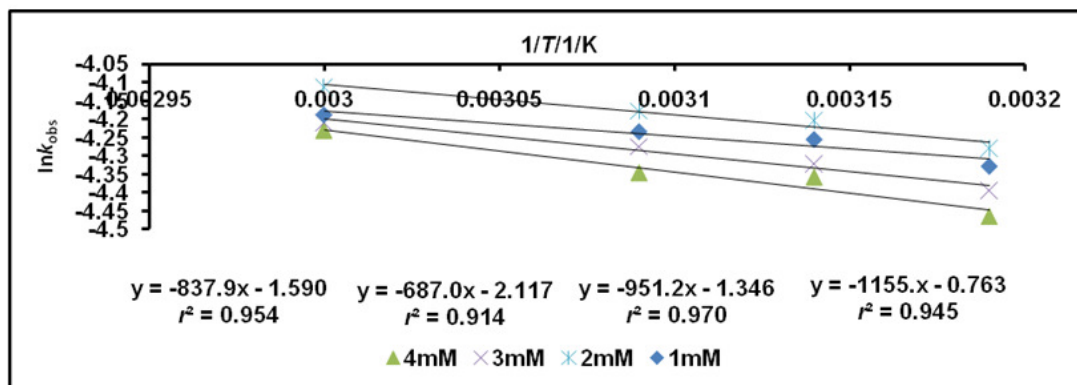
Fig. 3. Arrhenius plots for the determination of activation energy for unfolding of the enzyme at different salt molar concentrations
