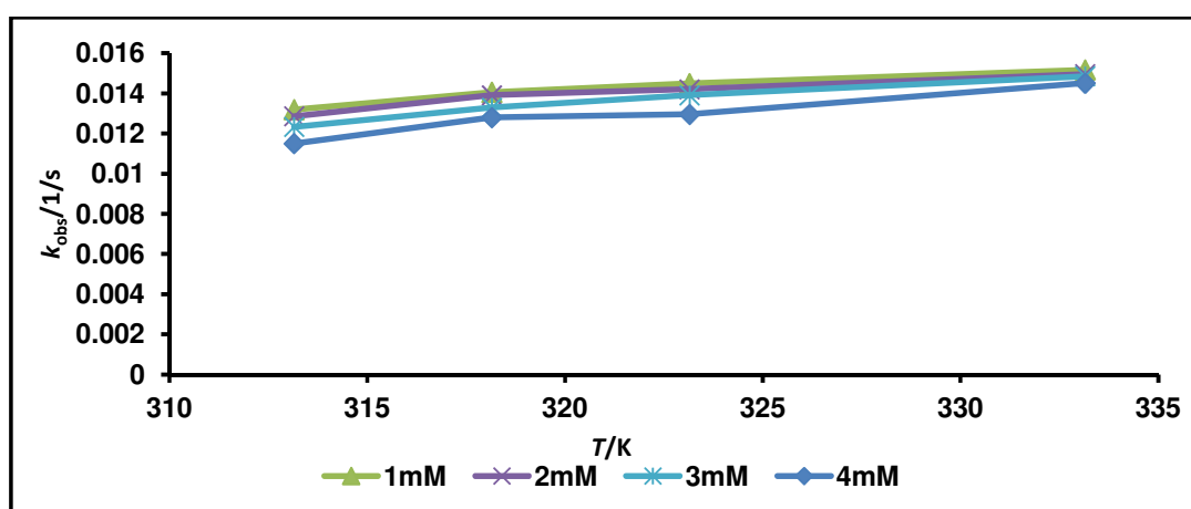
Fig. 1. Plot of apparent rate ( k_{obs} ) versus absolute temperature ( T ) showing the trend of k_{obs} with increasing T at different molar concentration of calcium chloride (▲), (×), (✱), and (◆) are assays and plots at 1 mM, 2 mM, 3 mM, and 4 mM respectively
