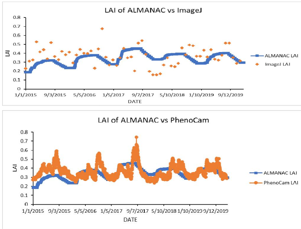
Fig. 9. Graphs of creosote bush from jersand comparing the LAI from ALMANAC with image analyses results (top) and then the LAI from ALMANAC with the transformed GCC from the PhenoCam website (bottom). The LAI values from ALMANAC using default plant parameters were not shown for this site due to simulation errors when they were used
