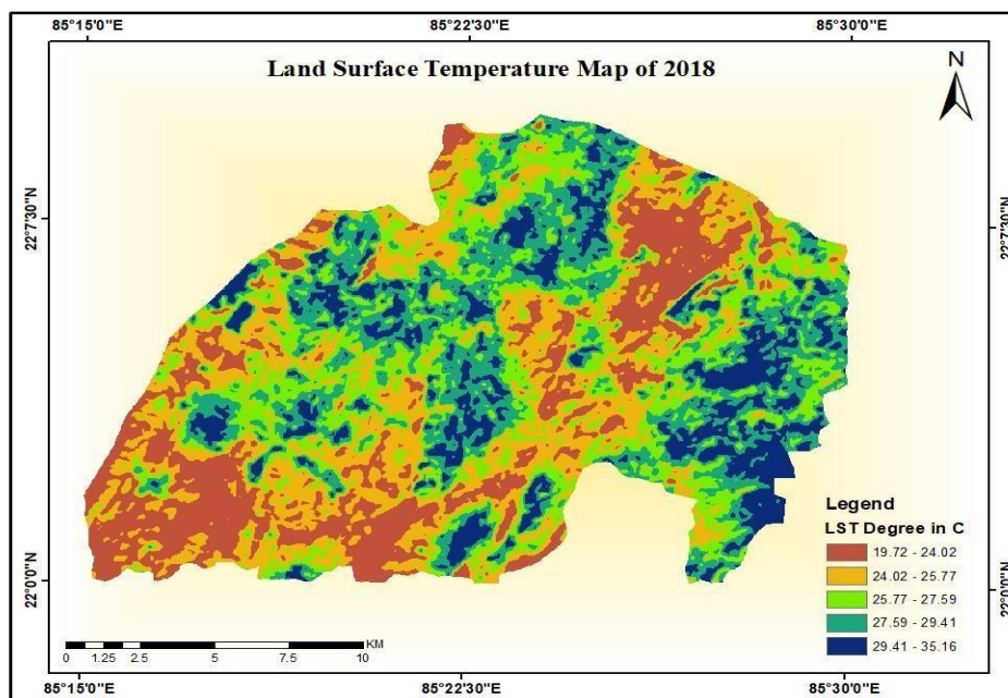
Fig. 16. Land surface temperature Map for the Year 2018 (Min Temperature 19.72°C, Maximum Temperature 35.16°C)
