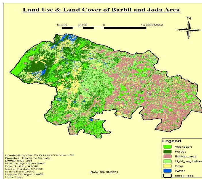
Fig. 7. The Land use and land cover Map of Joad and Barbil area, Odisha
