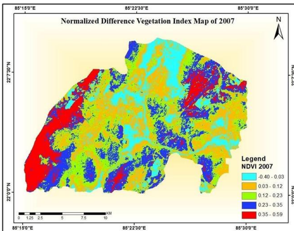
Fig. 17. NDVI Map of Joda Barbil area for the Year 2007
