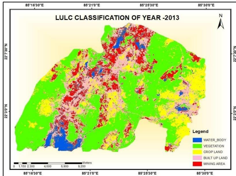
Fig. 13. LULC classification Joda area of LISS IV in the year 2013, (LISS III data)
