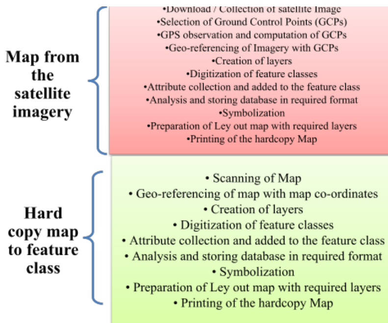
Fig. 10. The map from the satellite imagery & the hard copy map to feature class
