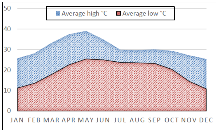
Fig. 8. The averaged high and low temperature of Joda area (GOO Masterplan -2030 [27]) The mean monthly temperature of the study with high and low temperatures are 30.77°C and 19.29°C respectively (Fig 8). The average annual rainfall is about 1378mm (Fig. 9)
