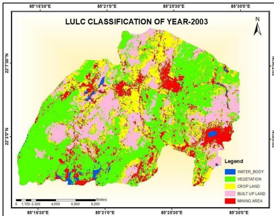
Fig. 11. LULC classification Joda area of LISS IV in the year 2003, (LISS III data)
