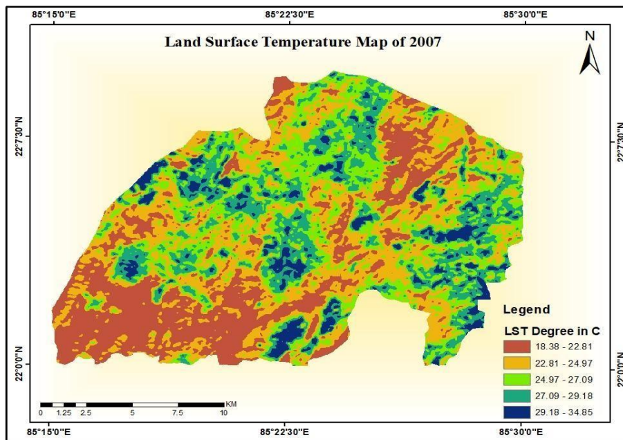
Fig. 15. Land surface temperature Map for the Year 2007 (Min Temperature 18.38°C, Maximum Temperature 34.85°C)
