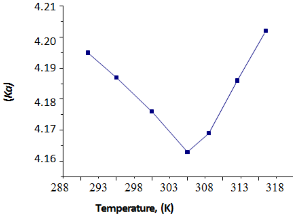
Fig. 2. The plot of K_a (thermodynamic dissociation constant) of benzoic acid into water against temperature (T) range
