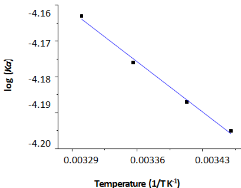
Fig. 3. The plot of K_a (thermodynamic dissociation constant) versus T (temperature) of benzoic acid into water
