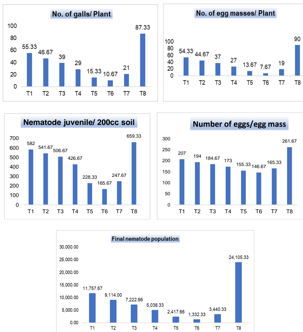
Fig. 2. Efficacy of newer nematicide on nematode reproduction in mung bean infected with root-knot nematode, M. Javanica
