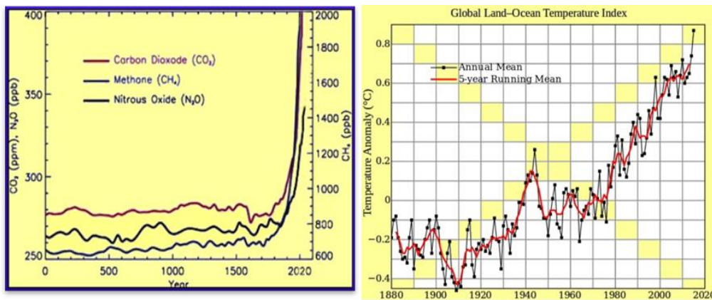
Fig. 1. Global Land Ocean temperature index
