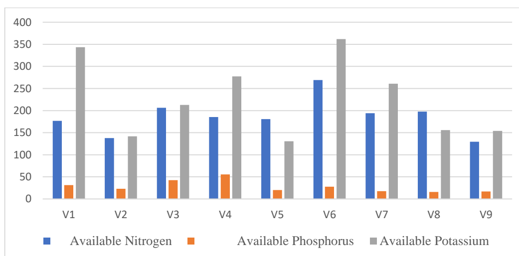
Fig. 7. Available Nitrogen (kg ha -1 ) Phosphorus (kg ha -1 ) Potassium (kg ha -1 ) of soil samples at 0- 15, 15-30, and 30-45 cm depth in various regions of different Taluk of Pathanamthitta district
