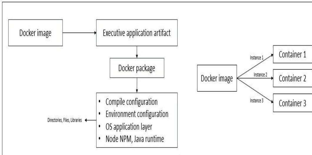
Fig. 4. Docker Image [43]
