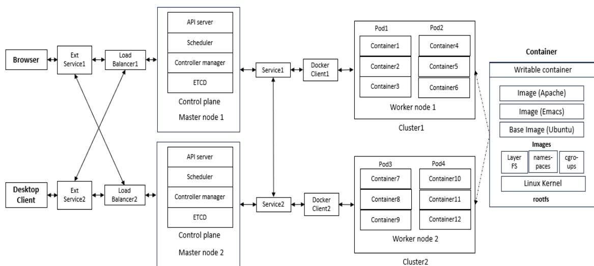
Fig. 1. Docker Architecture [43]
