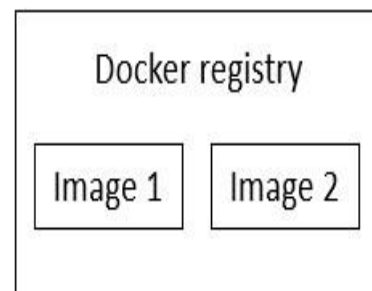
Fig. 5. Docker Registry [43]
