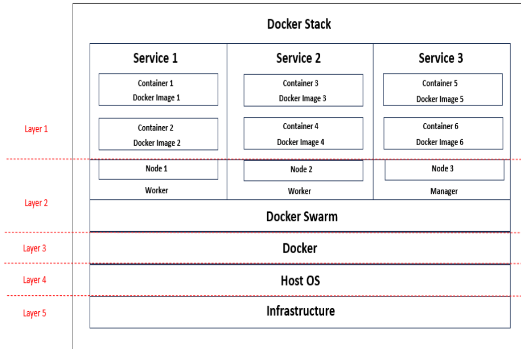
Fig. 10. Docker Stack [43]
