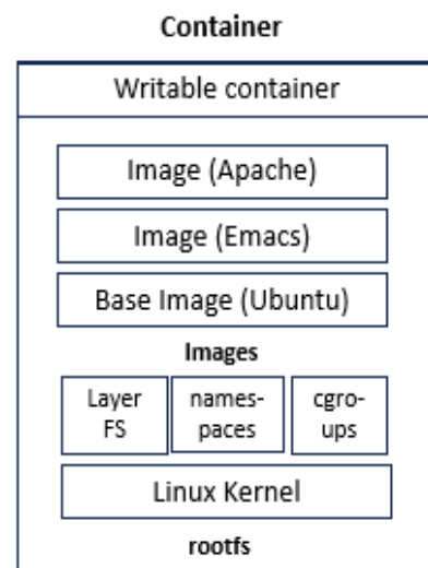
Fig. 3. Docker Container [43]
