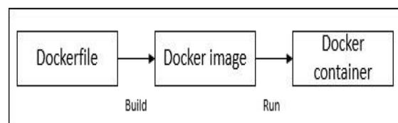
Fig. 8. Docker File [43]
