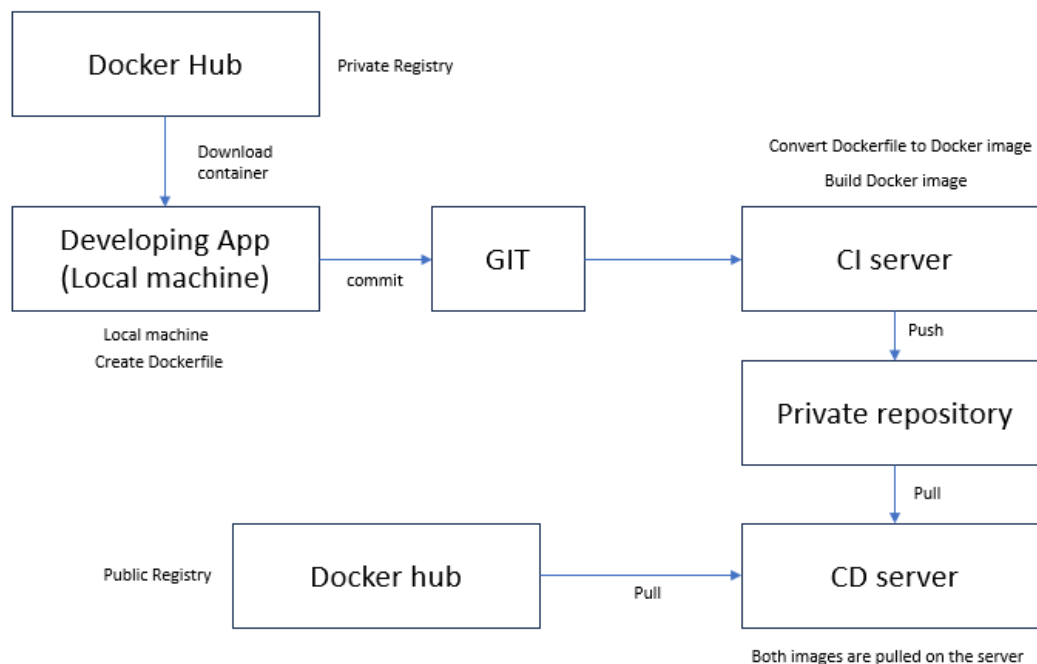
Fig. 11. Docker Deployment Process [43]
