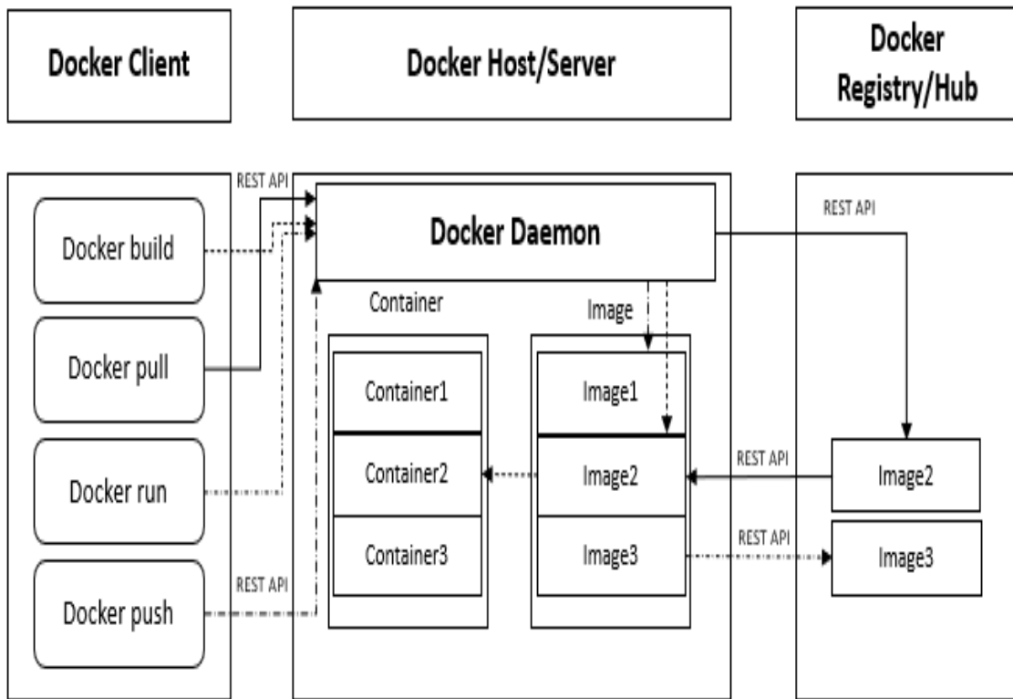
Fig. 2. Docker Client Server Architecture [43]
