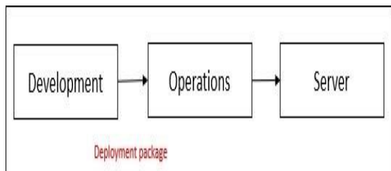
Fig. 9. Deployment Server [43]
