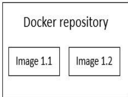
Fig. 6. Docker Repository [43]
