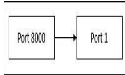
Fig. 7. Port Binding [43]
