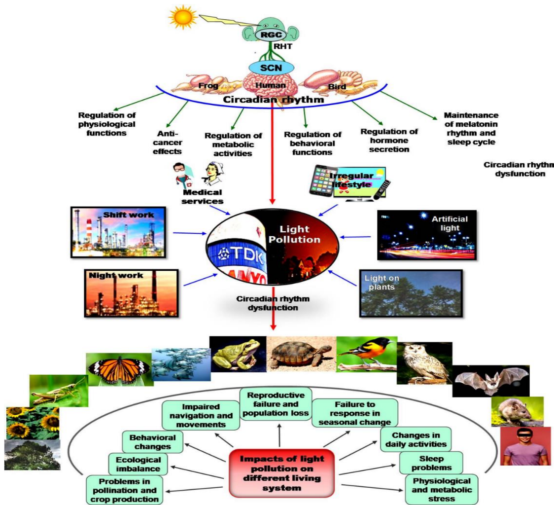
Fig. 2. Anthropogenic activity, sources of artificial light at night and effects of light pollution on living systems
