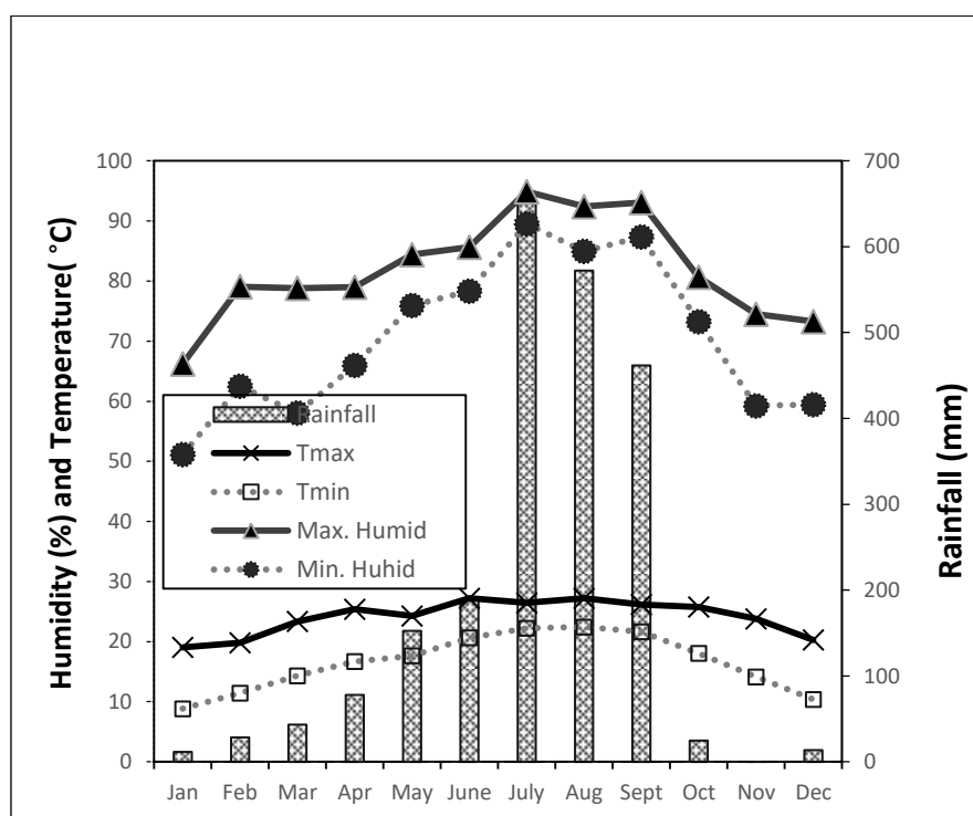
Fig. 1. Meteorological observations during the entire crop growth period
