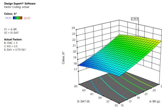
Fig. 6. Interaction effects of BR and DAT on b*
