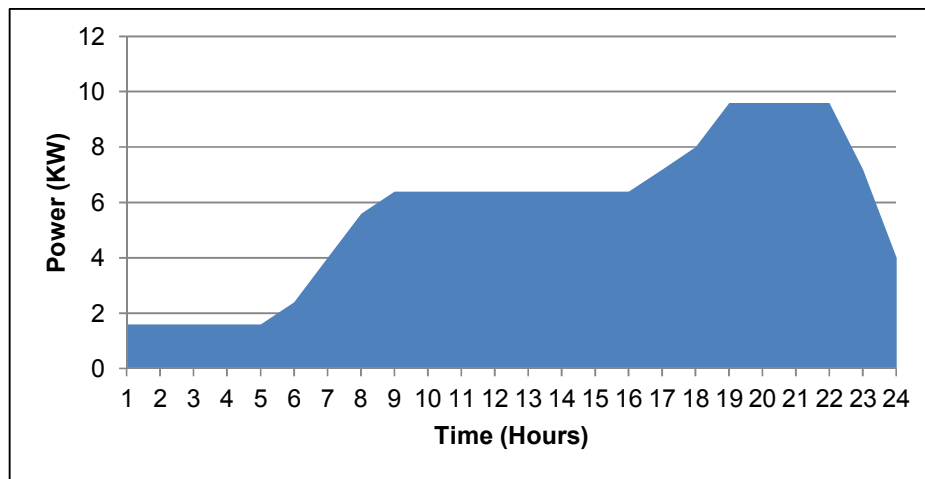
Fig. 4. Hourly load profile of Patar Char
