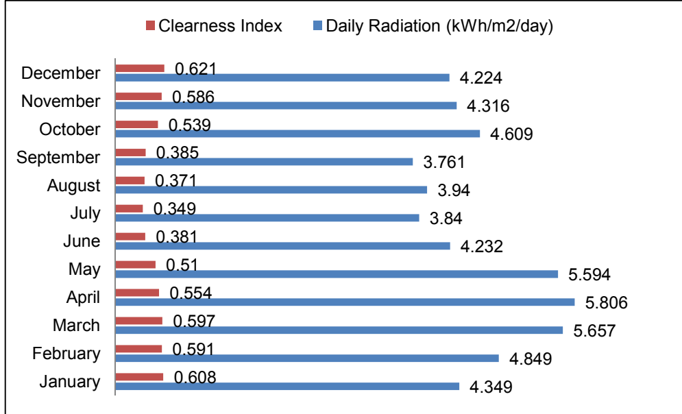
Fig. 5. Monthly solar radiation and clearness index of Patar Char
