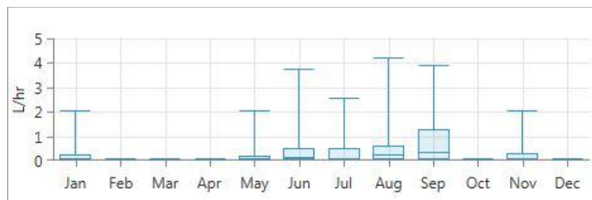
Fig. 6. Average fuel consumption intensity of diesel generator
