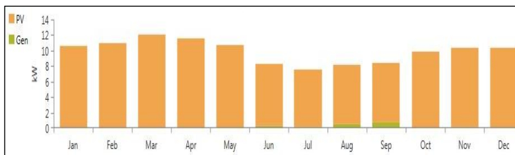
Fig. 7. Average monthly electricity production of Case A
