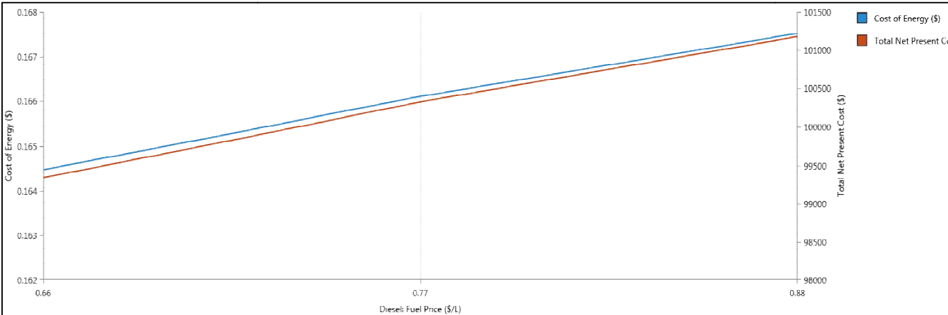
Fig. 9. COE and TNPC with the price of diesel
