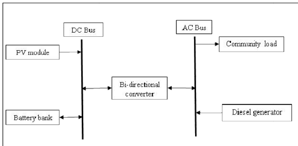
Fig. 1. Proposed block diagram of the off-grid hybrid energy system
