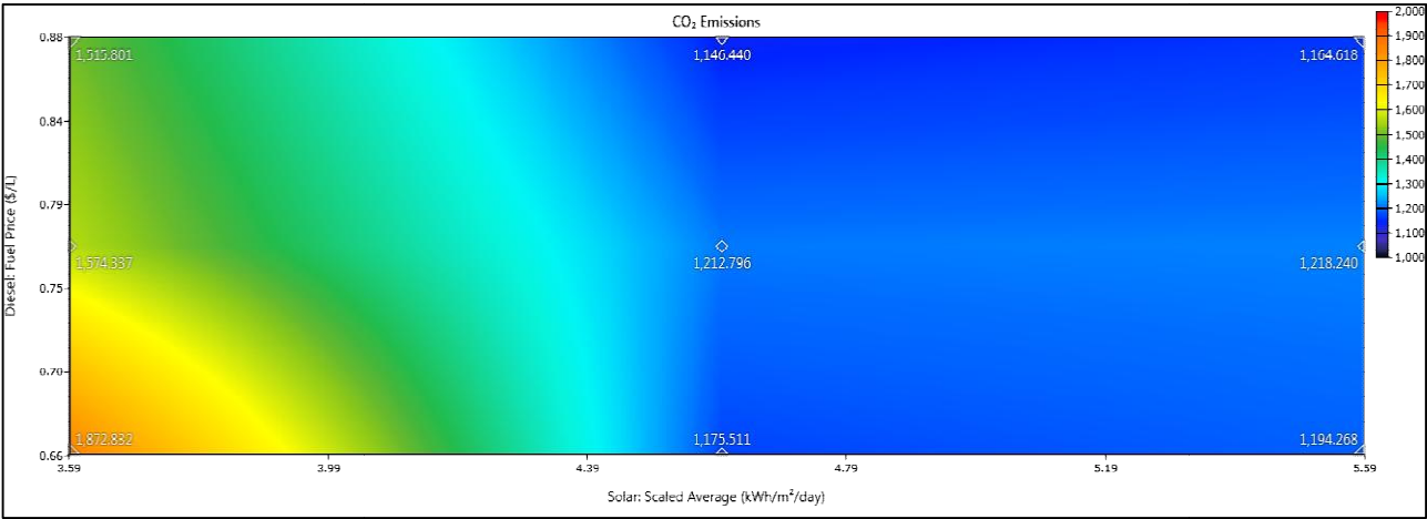
Fig. 12. CO 2 emissions with solar radiation and the price of diesel
