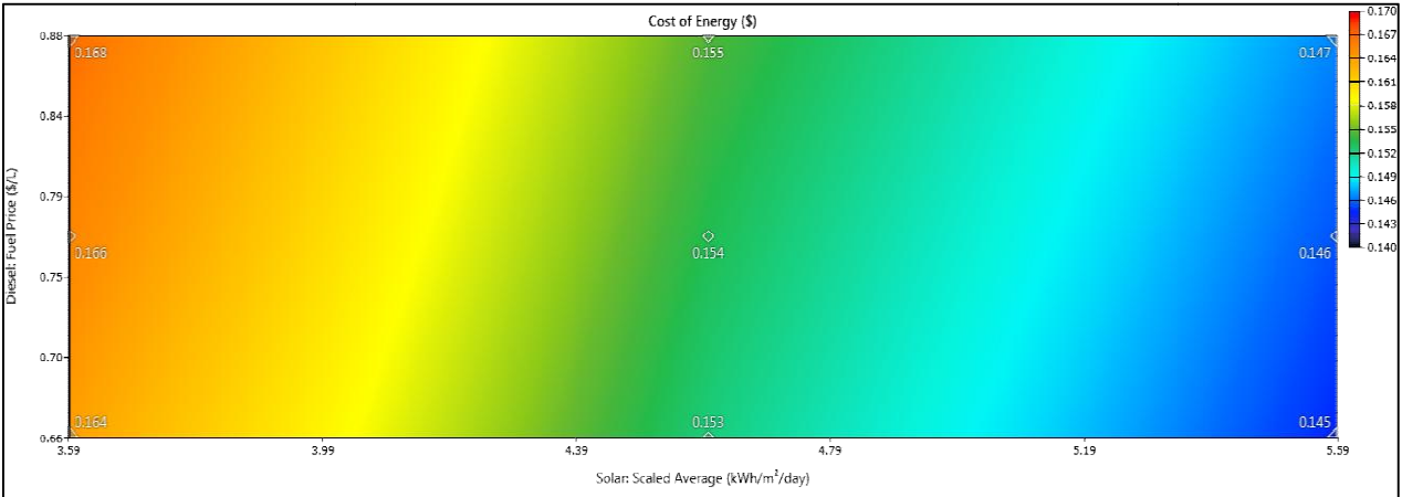
Fig. 11. COE with solar radiation and the price of diesel
