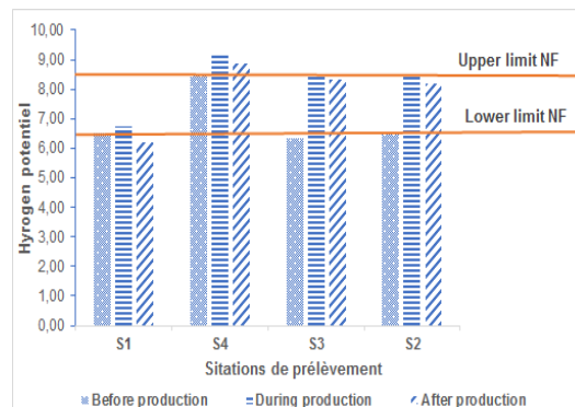
Fig. 4. PH variation
