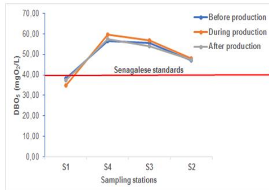
Fig. 10. BOD 5 content variation
