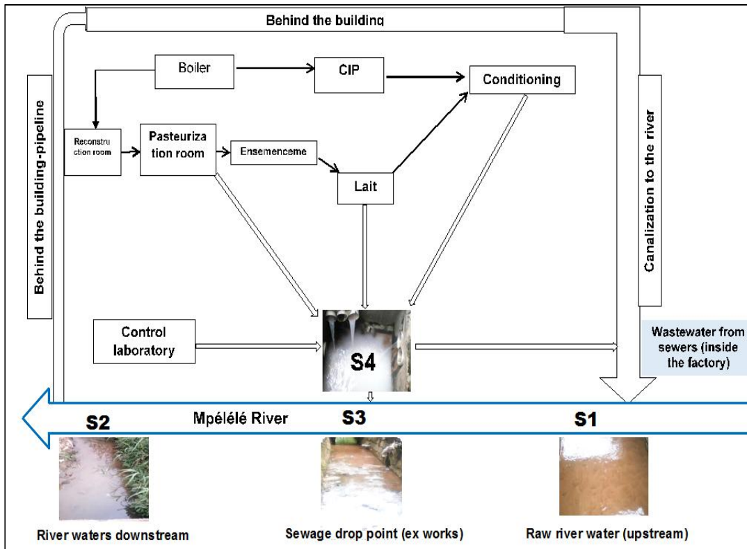
Fig. 2. Diagram of a part of the Bayo dairy installations and location of sampling stations
