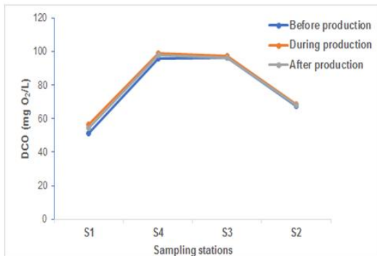
Fig. 9. Variation in COD content
