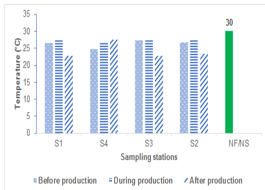
Fig. 3. Temperature variation
