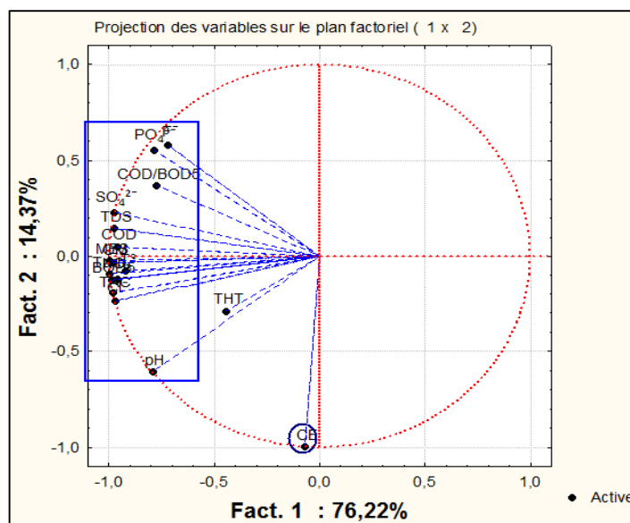
Fig. 13. Correlation of physicochemical parameters in the factorial plane (F1 x F2)
