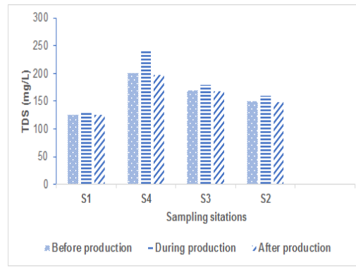
Fig. 6. Variation in TDS contents
