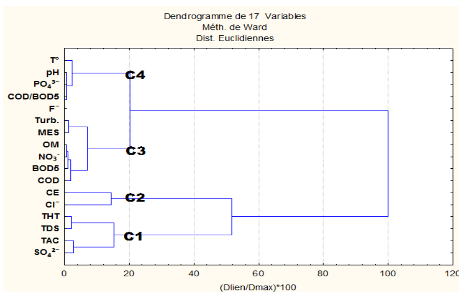
Fig. 14. Dendrogram for the classification of physicochemical parameters
