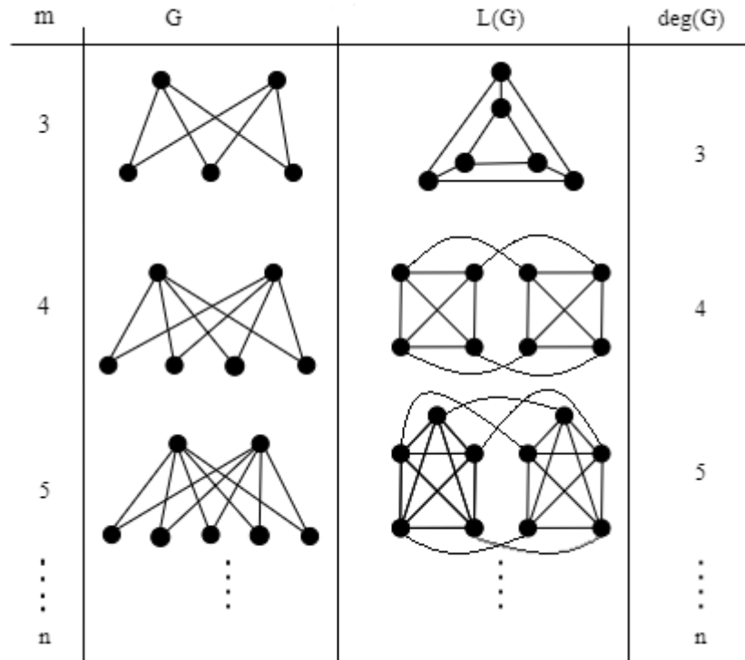
Fig. 6. Bipartite graph and corresponding line graph for fix n = 2
