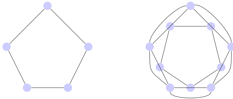
Fig. 3. C_5 graph and its total graph T(C_5)
