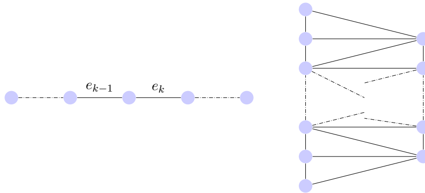
Fig. 4. P_n graph and the corresponding total graph T(P_n)
