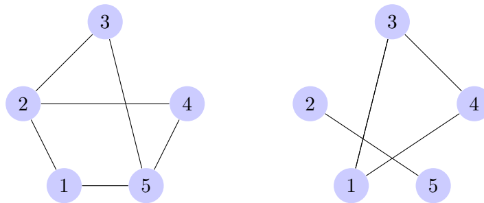
Fig. 1. A Graph and its complement
