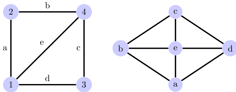
Fig. 2. A Graph G and the corresponding line graph L(G)
