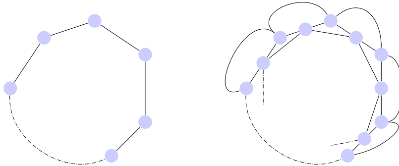
Fig. 5. C_n graph and the corresponding total graph T(C_n)
