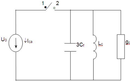
Fig. 1. Scheme for analyzing the current passing through the arc
