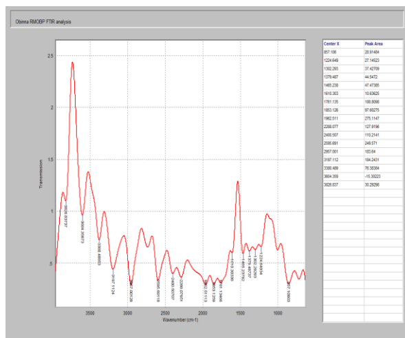
Fig. 1. FTIR spectra of raw OBP
