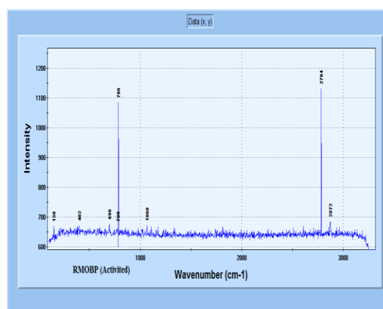
Fig. 4. RAMAN spectra of MCC
