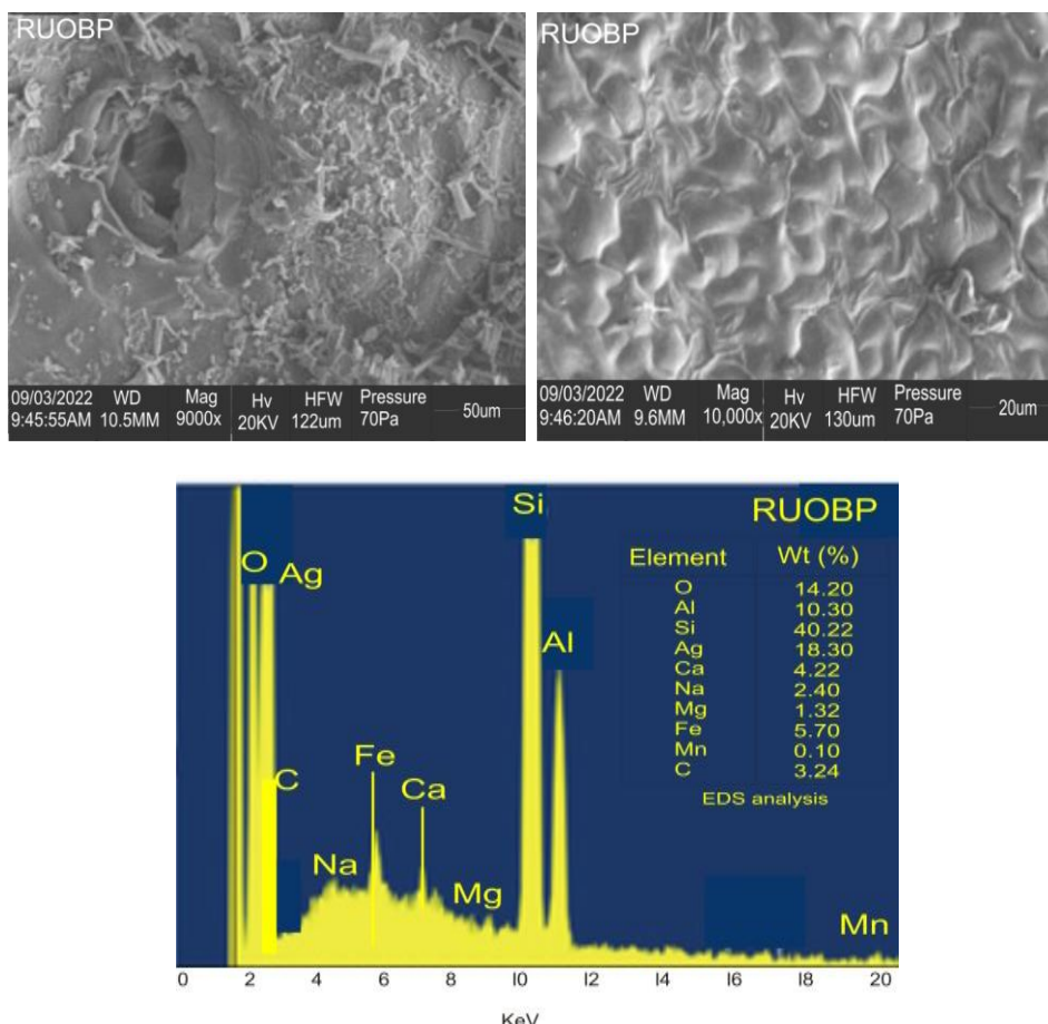
Fig. 5. SEM Micrograph and EDS Analysis for Raw OBP
