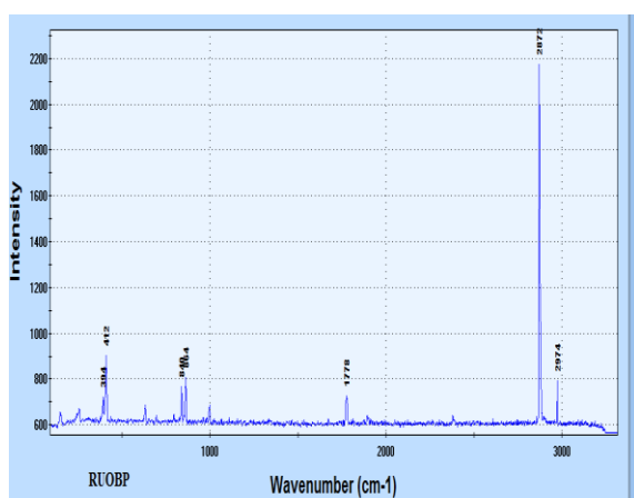
Fig. 3. RAMAN spectra of raw OBP
