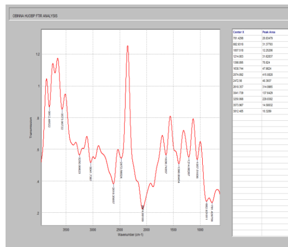
Fig. 2. FTIR spectra of MCC
