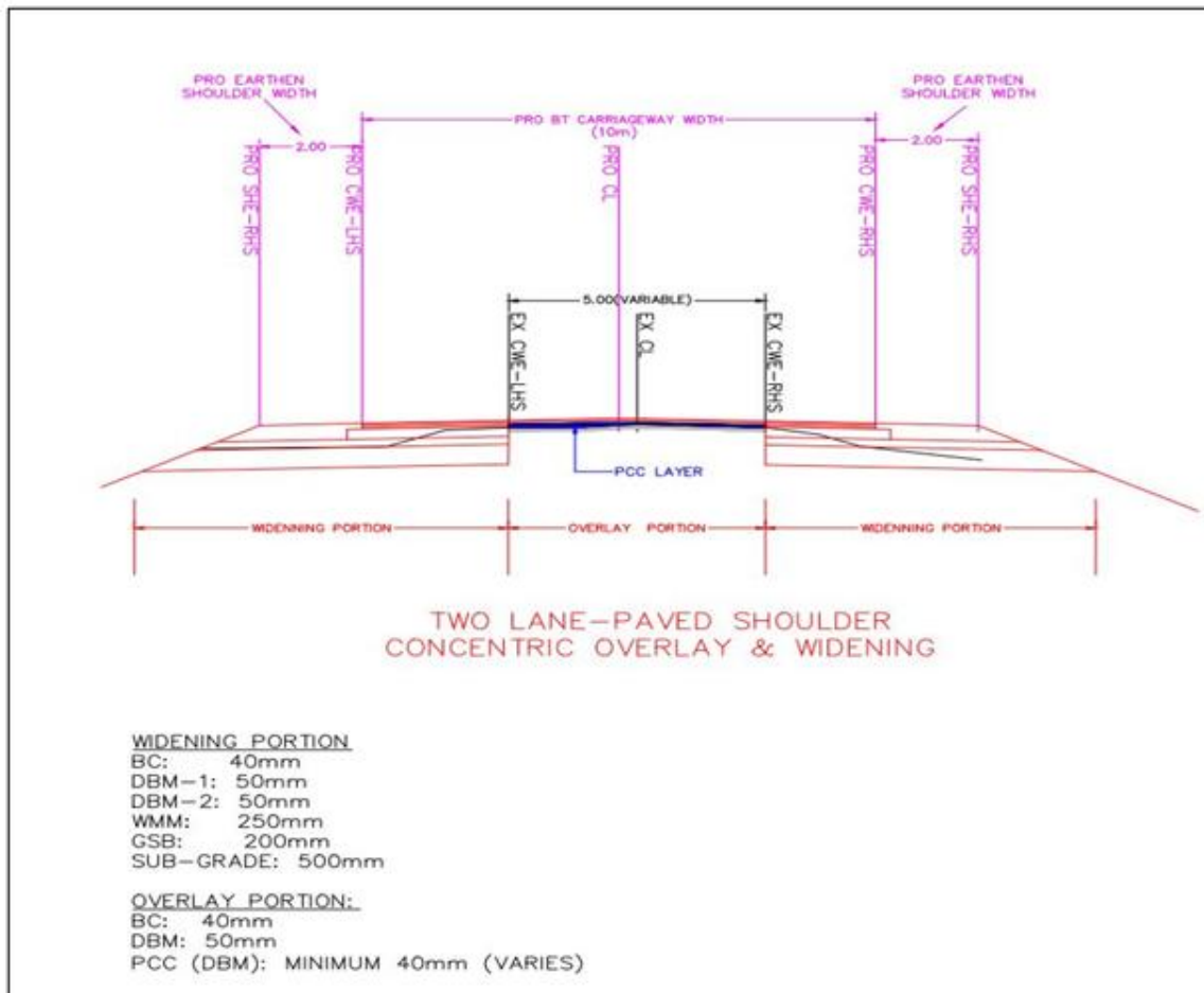
Fig. 6. TCS drawing for overlay & widening of flexible PAVEMENT
