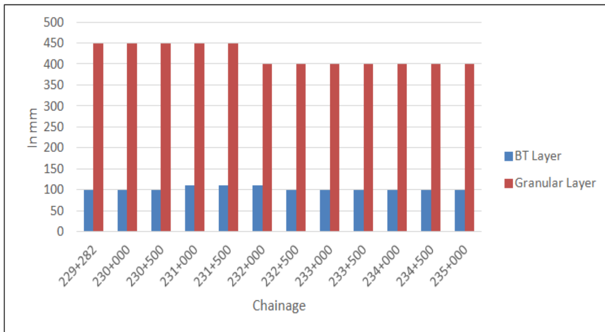
Fig. 4. Existing pavement layer thickness
