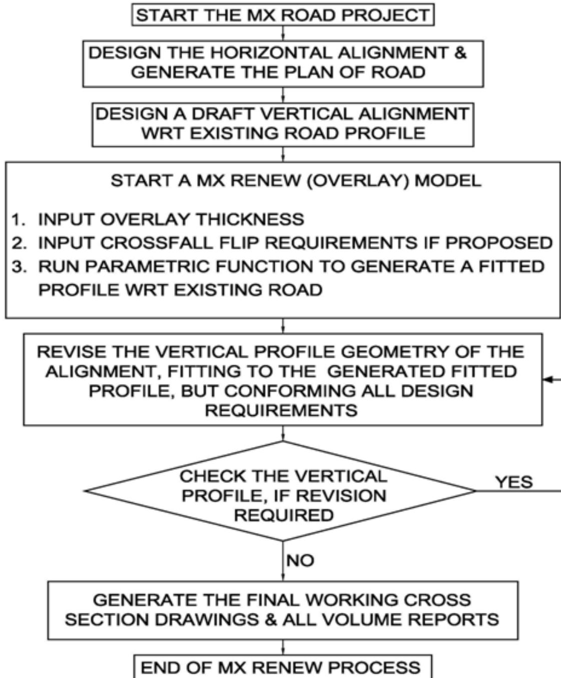
Fig. 10. Flow chart showing Overlay Design Process in MX Road
