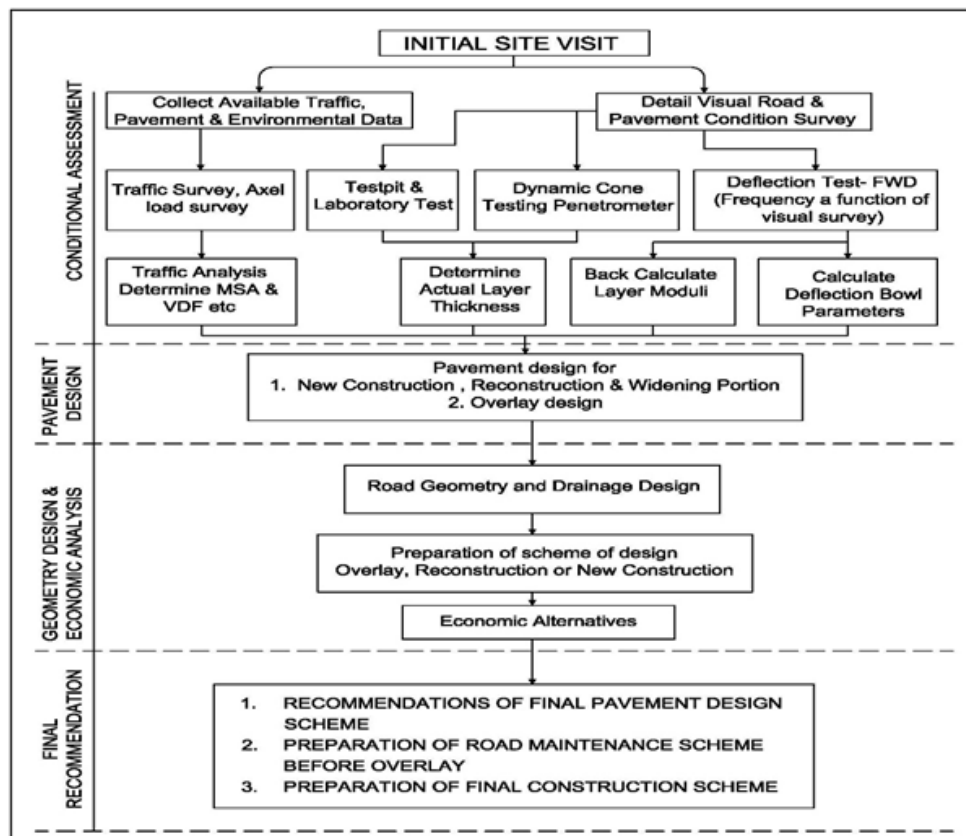
Fig. 3. Flow chart for overlay design of road
