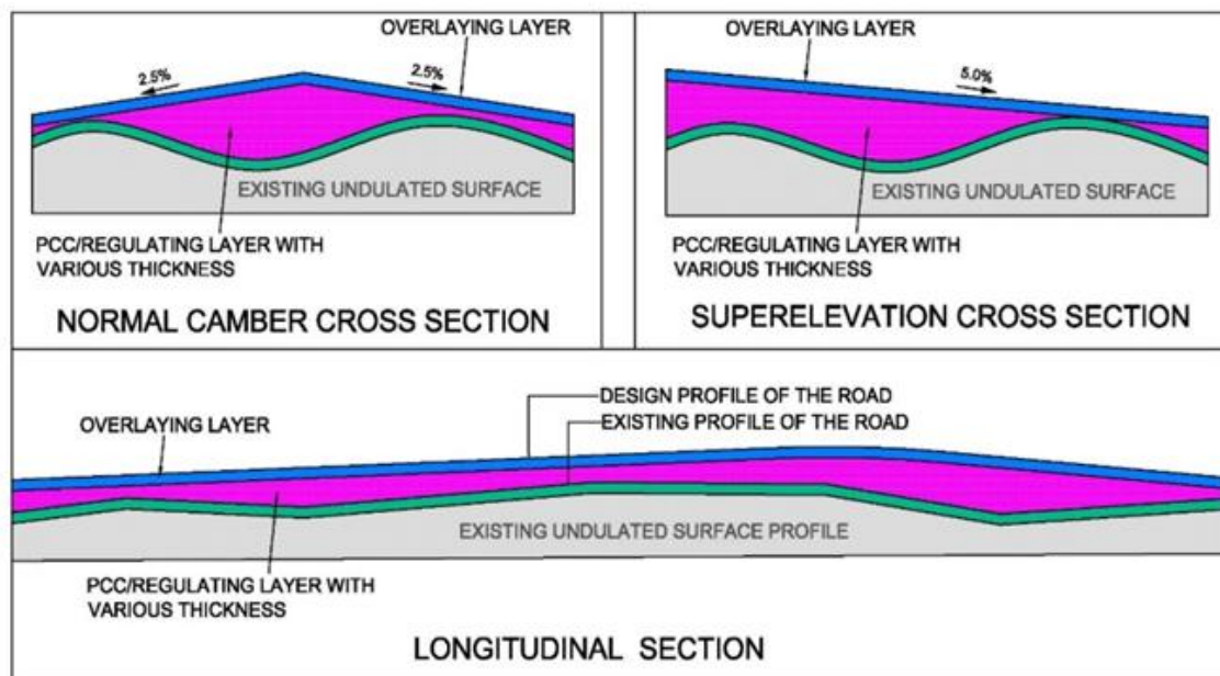
Fig. 1. Scheme of road overlay
