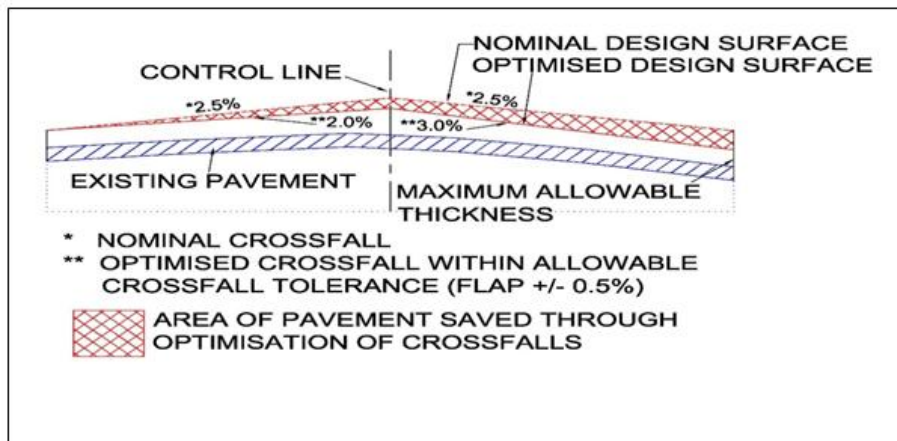
Fig. 9. Optimized design cross section
